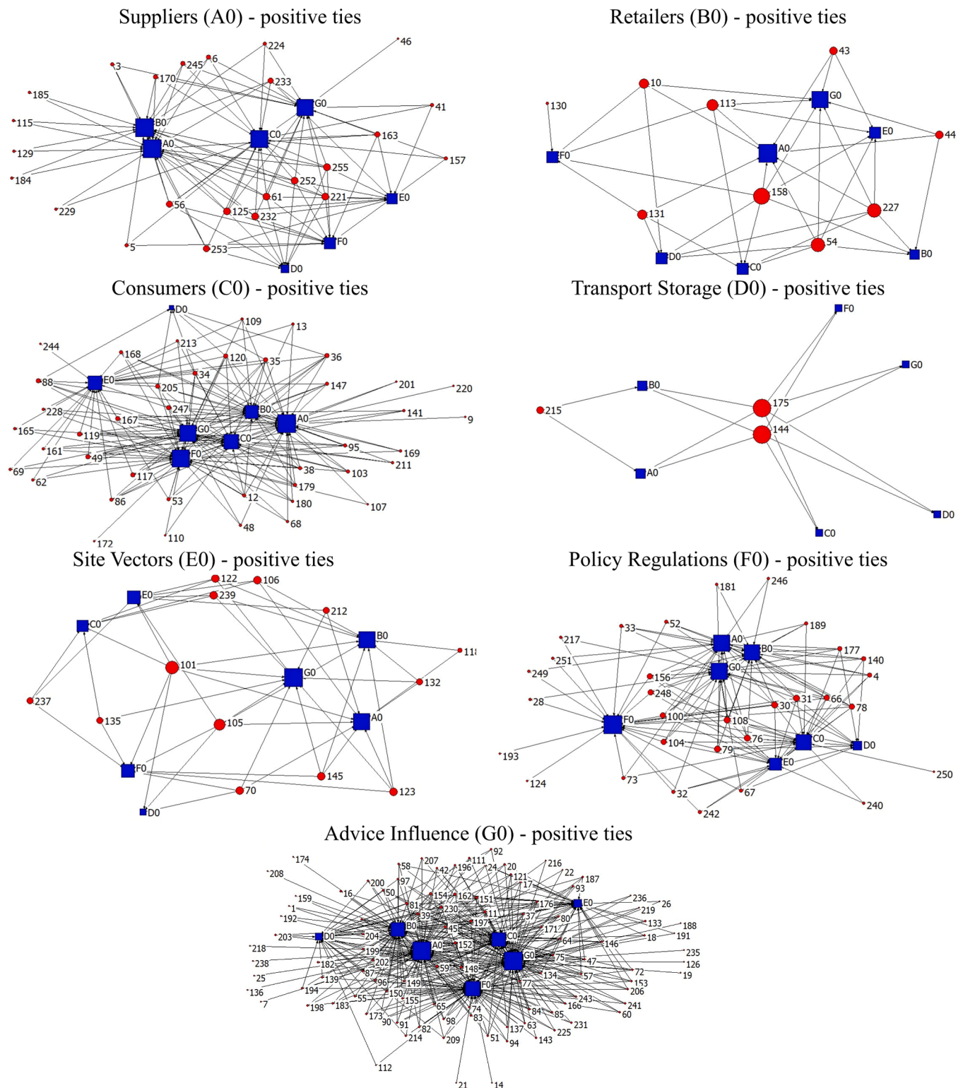
Fig. 3. Networks of positive collaborations between stakeholders by category. Red circles are the individual stakeholders (with respective numeric ID) involved in the survey that belong to the reference category. Blue circles are the other stakeholder categories indicated by the individual stakeholders. The size of the shapes refers to the centrality values (larger circles correspond to higher centrality values), while the lines are the ties.
